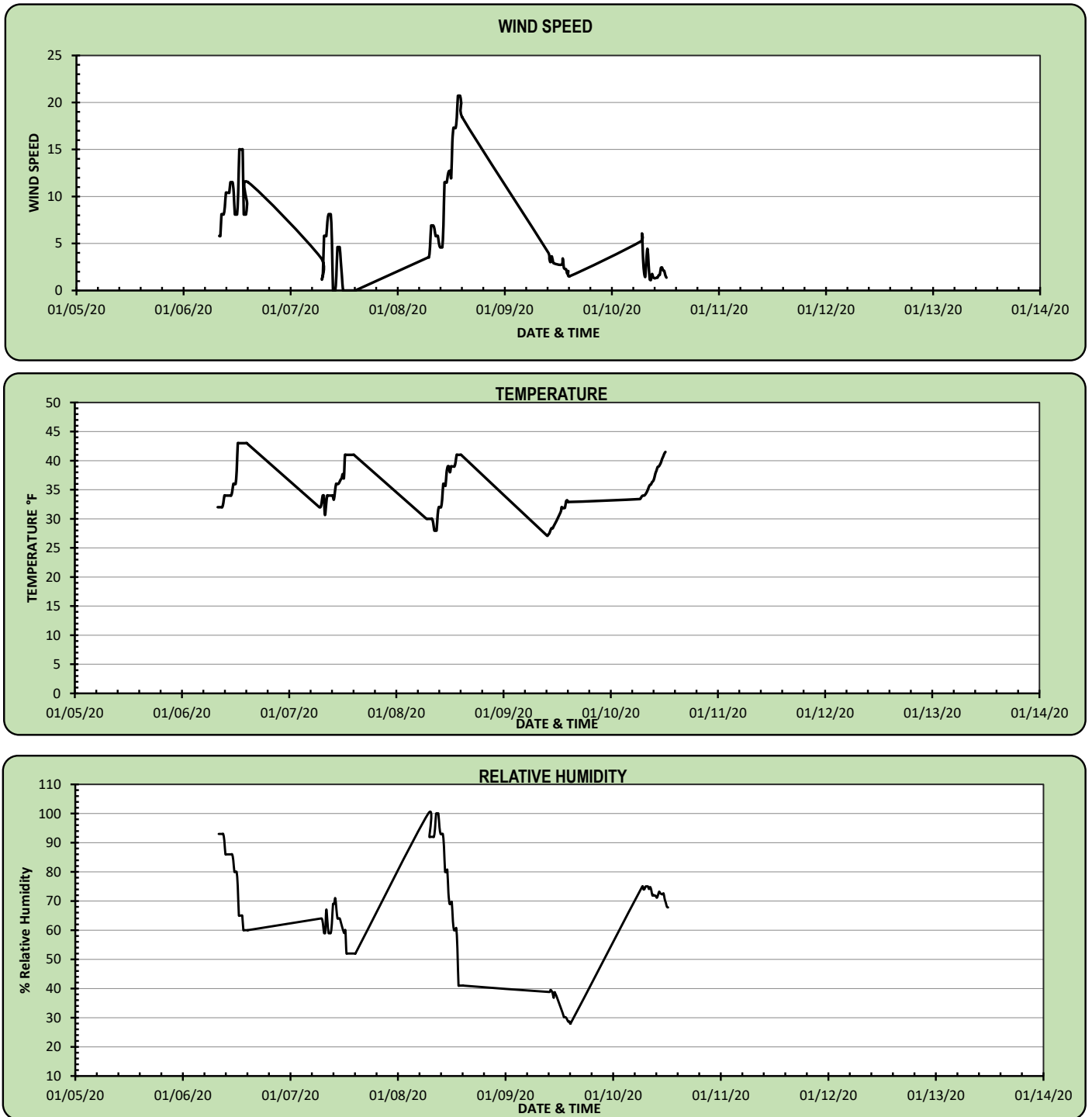
Figure 1: Meteorological Data
