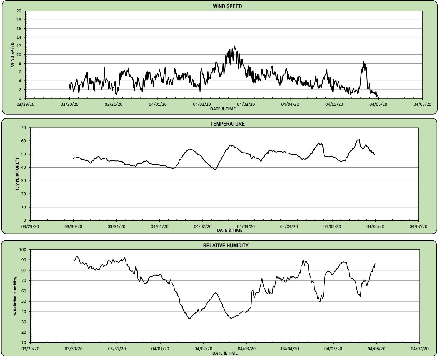
Figure 1: Meteorological Data
