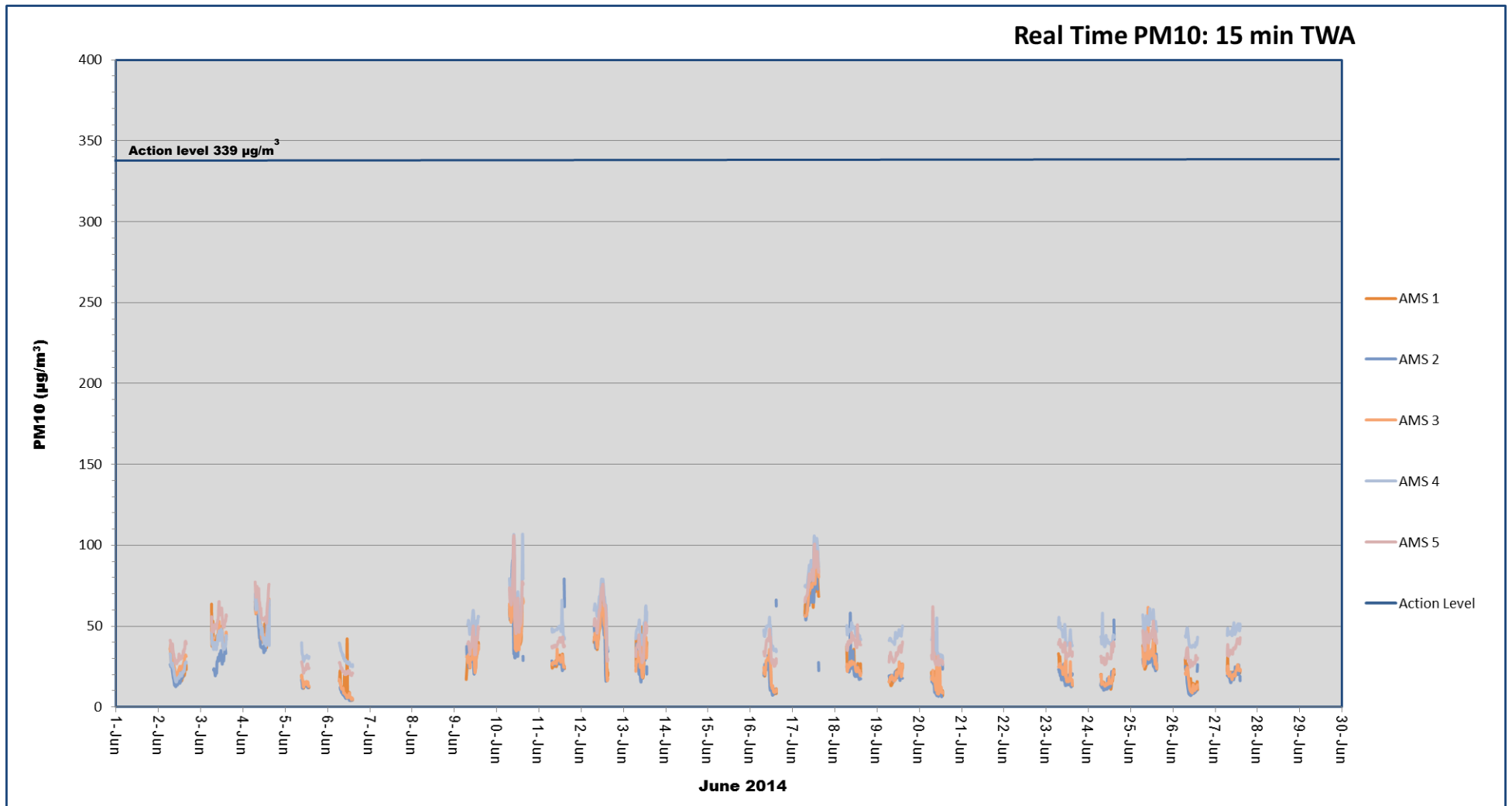
Figure A- 1: Real-Time 15-minute average PM 10 Monitoring Results
